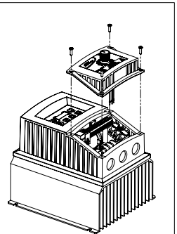
Figure 3: Replace Potentiometer as SMV Terminal Cover
